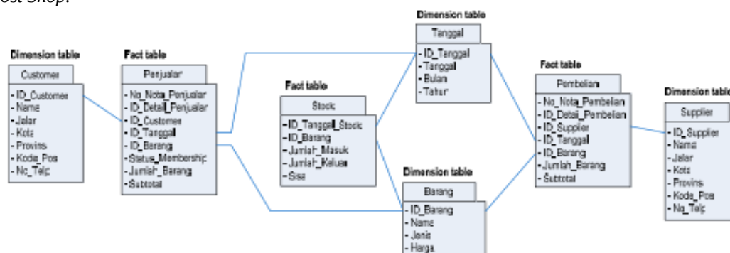
Gambar 11. Fact Constellation Schema Post Shop
