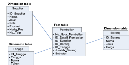
Gambar 6. Star Schema Pembelian Post Shop
