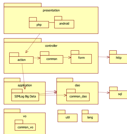
Gambar 3. Component Diagram
