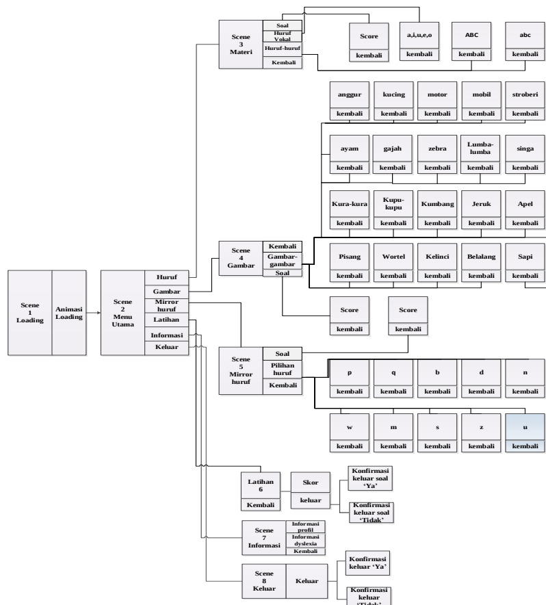
Gambar 7. Flowchart View
