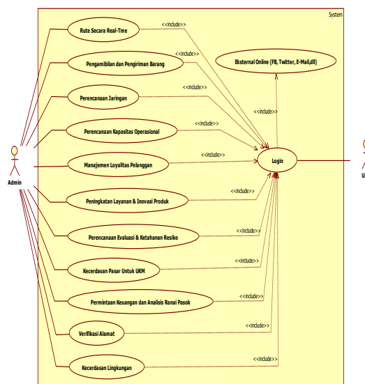
Gambar 2. Usecase Diagram
