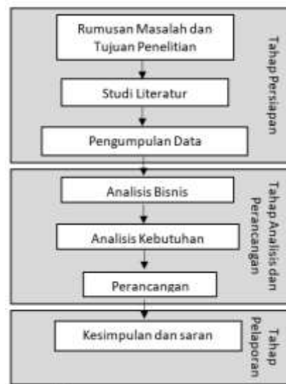
Gambar 1. Metode Penelitian
