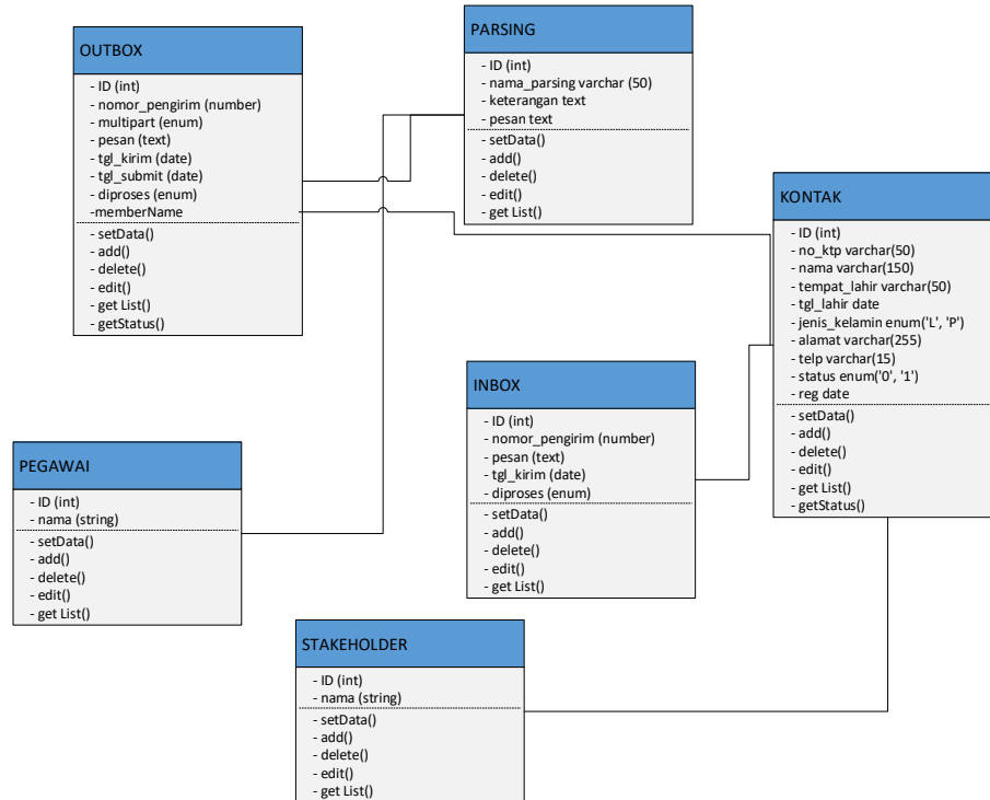
Gambar 2 Class Diagram Smart System Service
