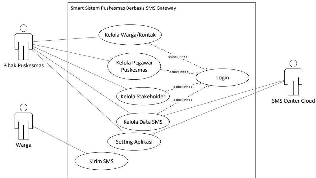
Gambar 1 Use Case Smart System Service
