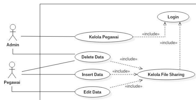
Gambar 3.4. Use Case Diagram File Sharing
