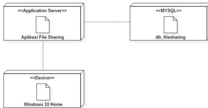
Gambar 3.5. Deployment Diagram
