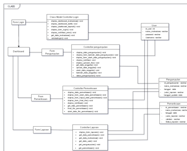
Gambar 9 Class Diagram
