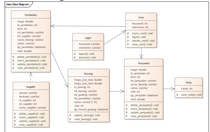
Gambar 7. Class Diagram
