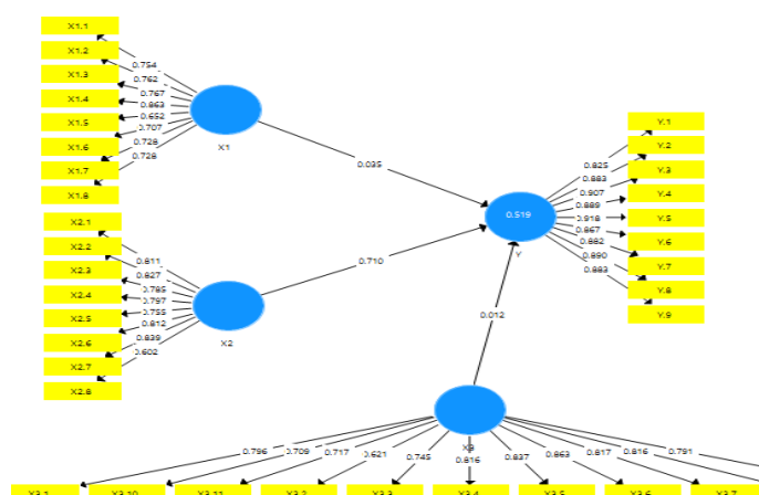
Gambar 1. Output Path Diagram
