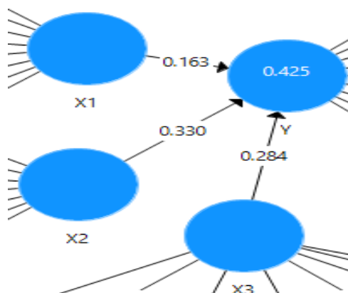
Gambar 2. Koefisien-koefisien Standardized Model Struktural
